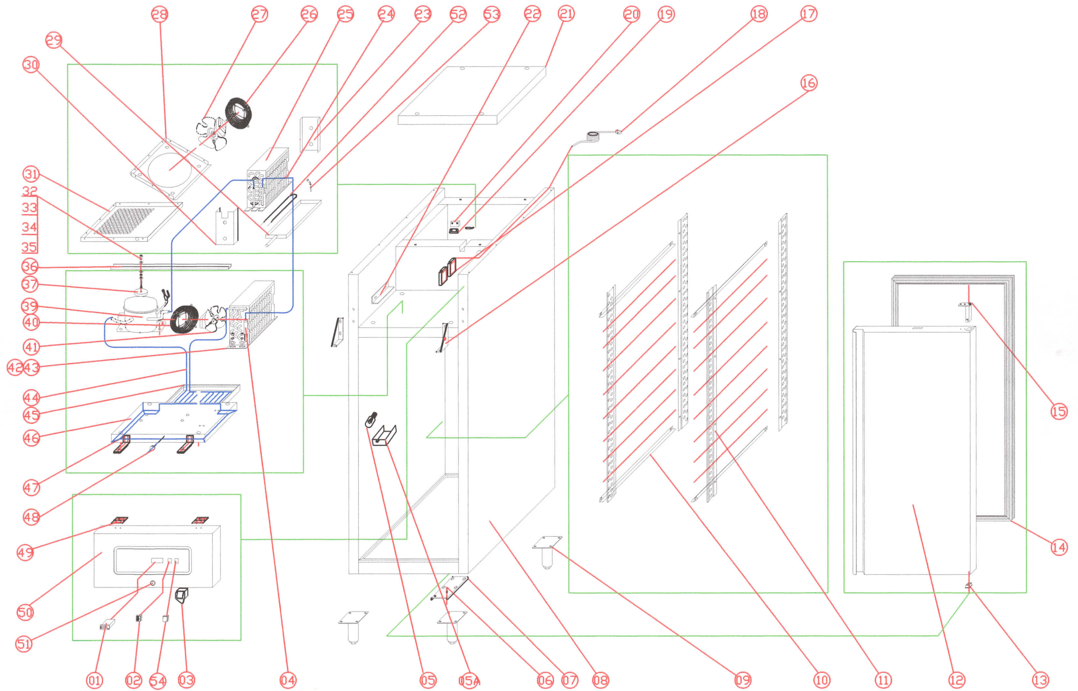
EXPLODE DIAGRAM OF PA800TNK(WITH H. E. )
