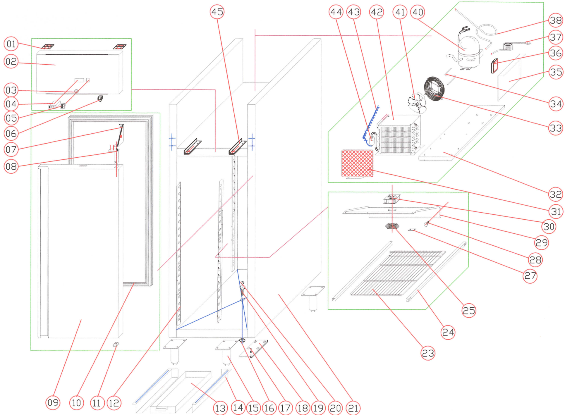
EXPLODE OF GN600BT (GN600BTZ0.6)
