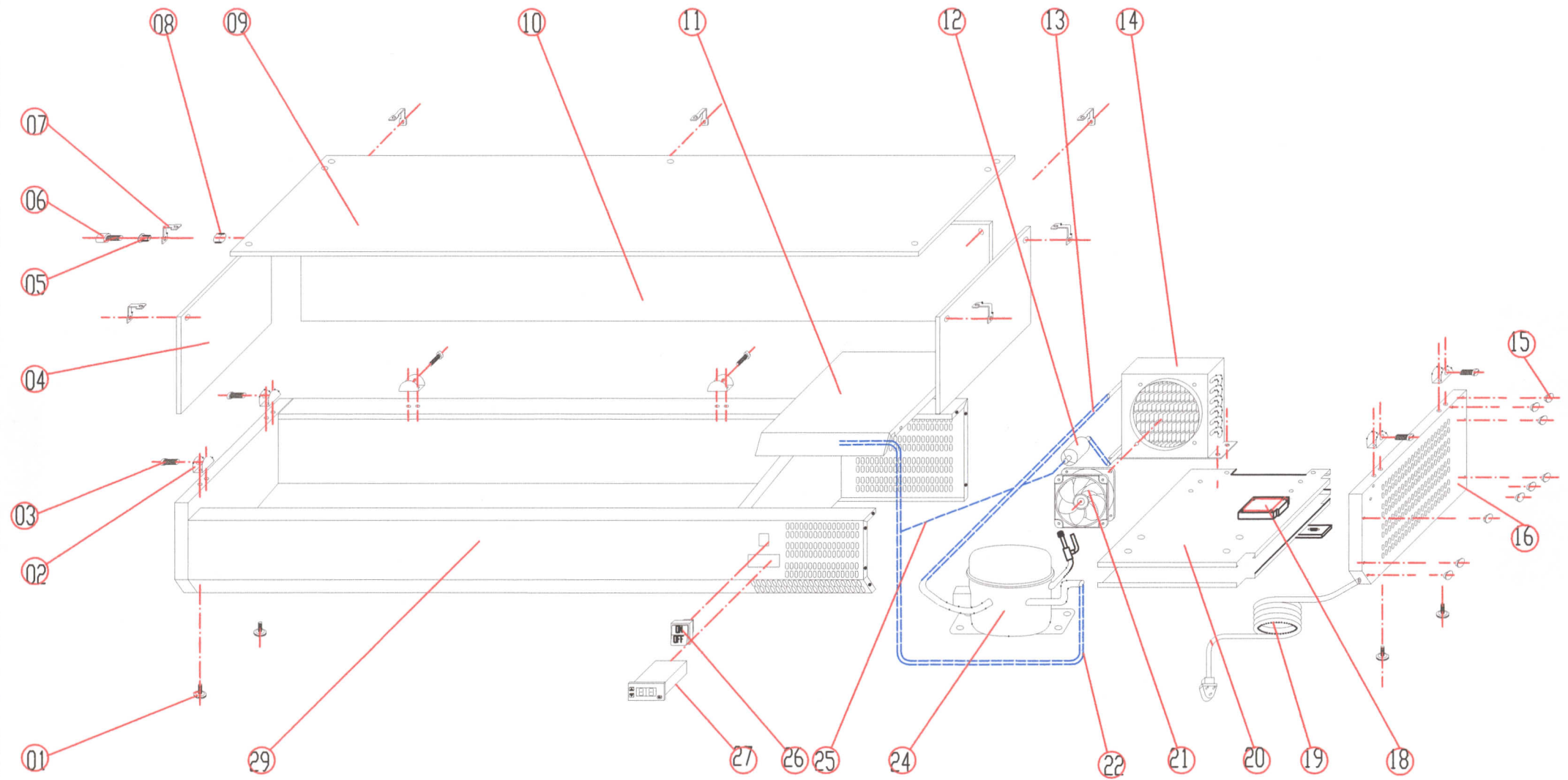
EXPLODE OF VRX1400/330
