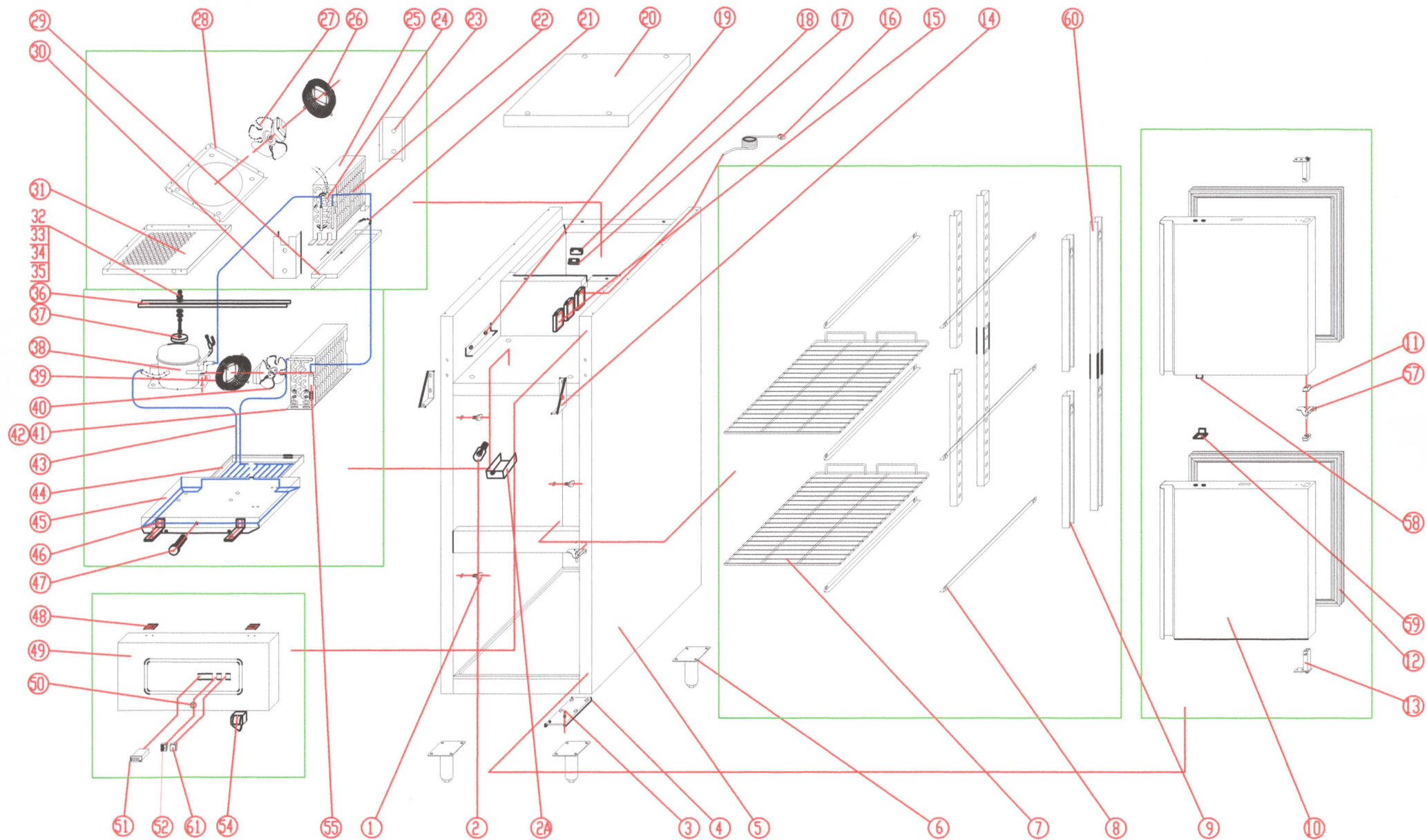
EXPLODE DIAGRAM OF GN650BTM
