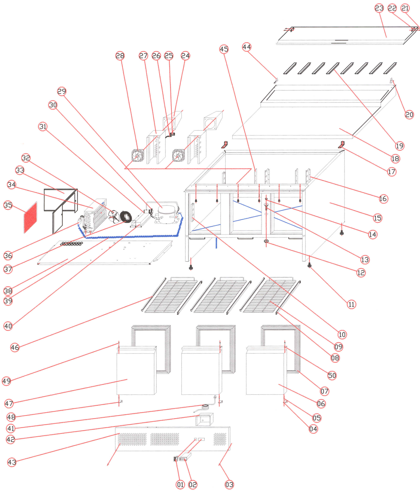
EXPLODE OF PS300GN1/6
