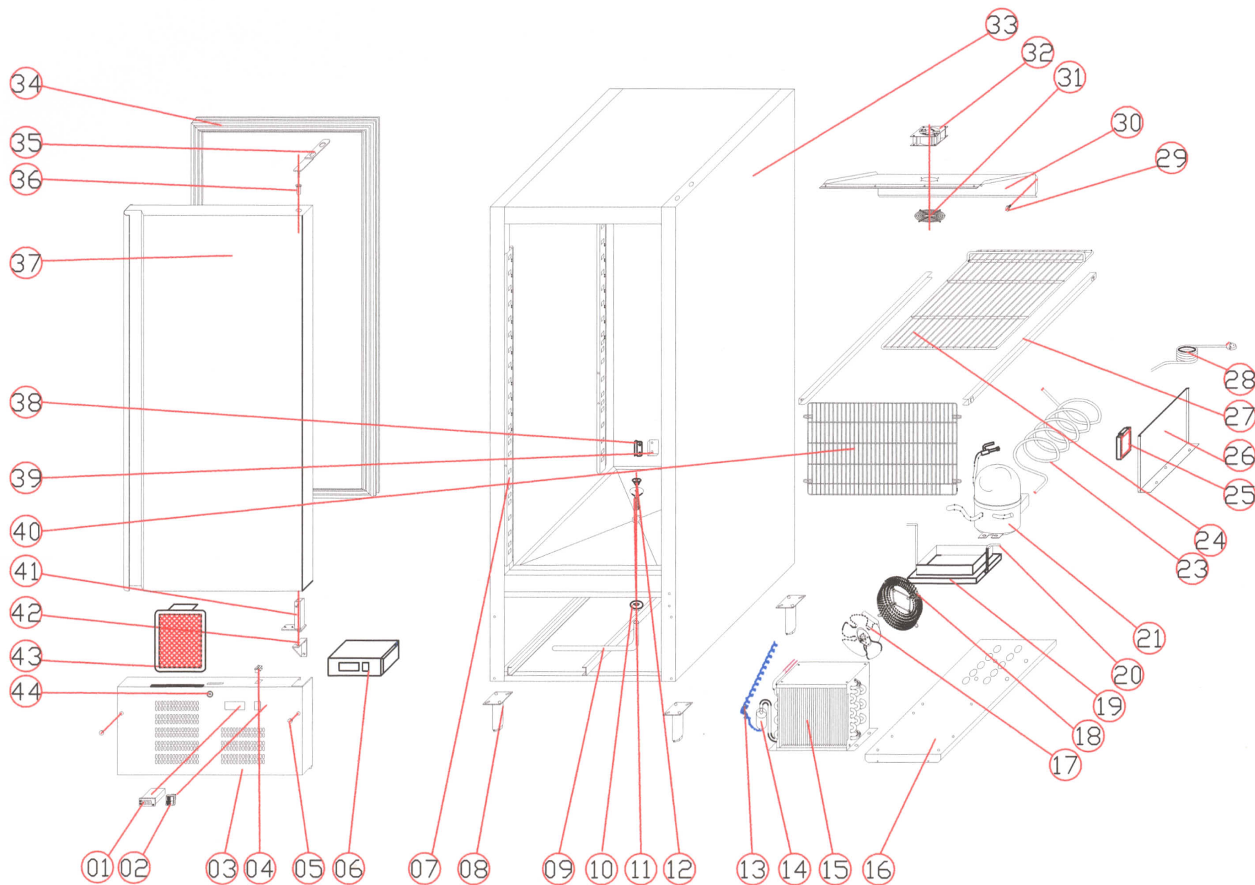
EXPLODE OF SNACK400STN
