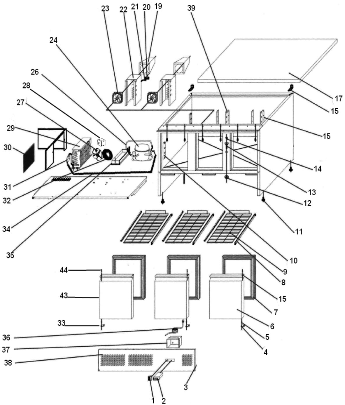
S901-S903 TOP EXPLODE OF S903PZ - SS45
