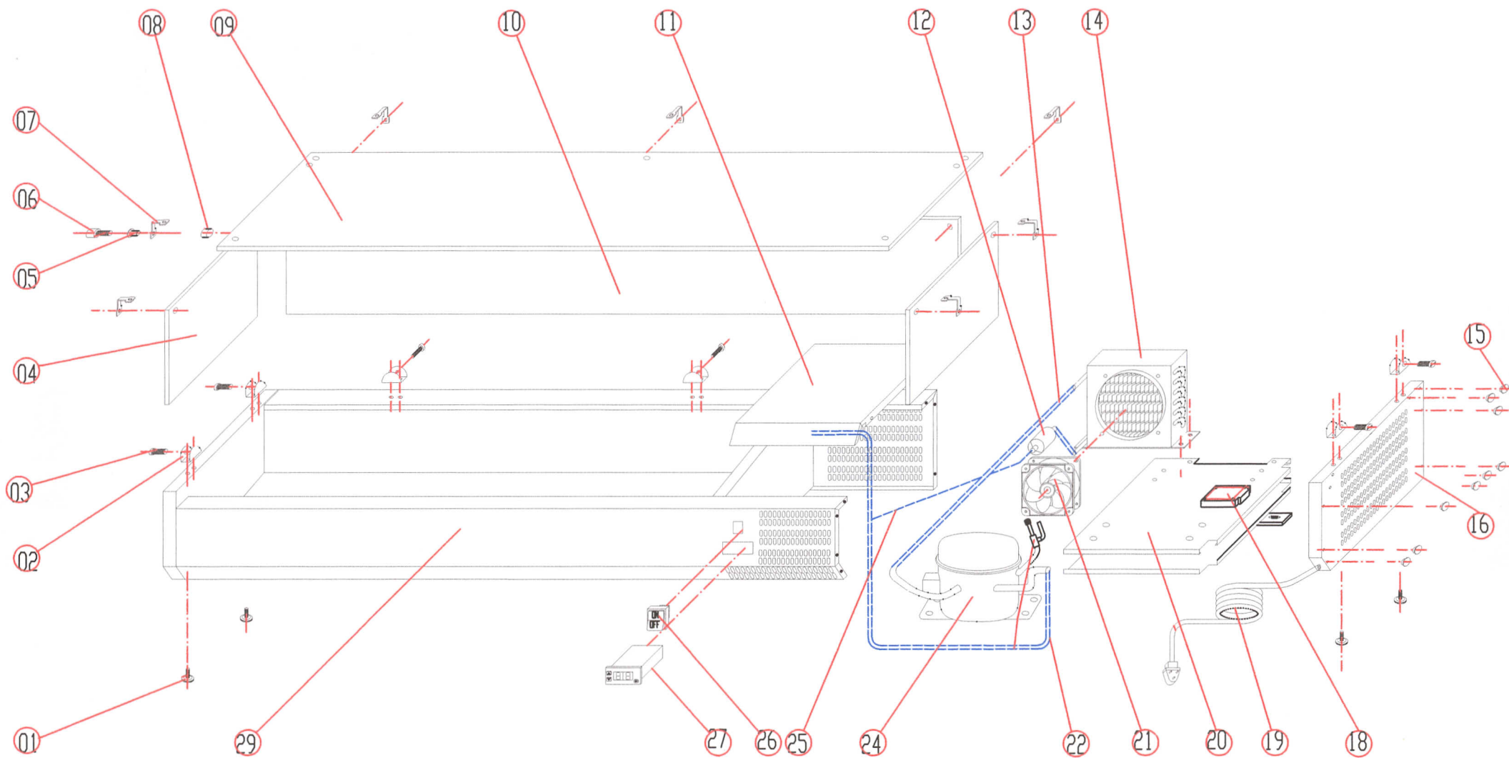
EXPLODE OF VRX1800/380
