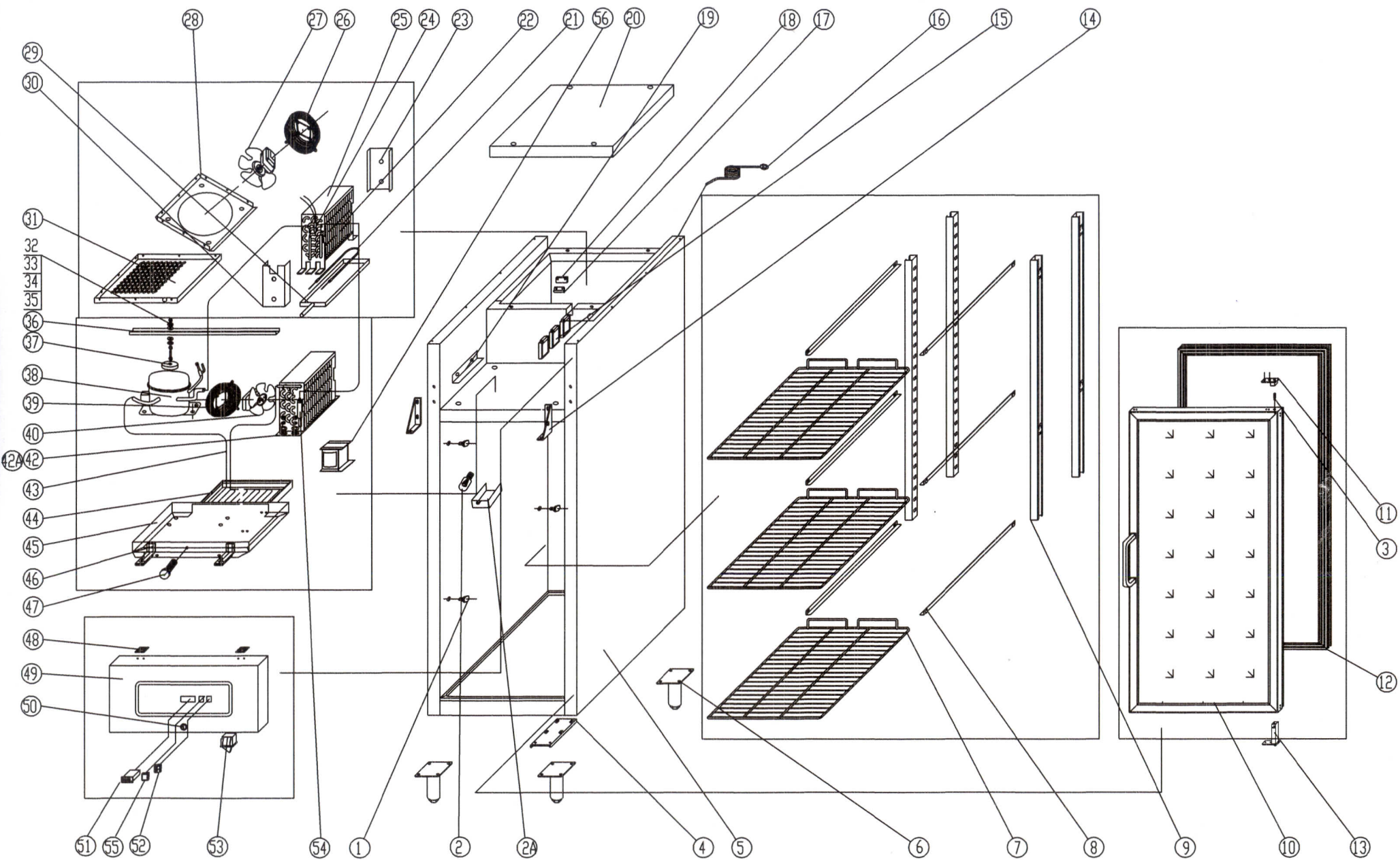
EXPLODE DIAGRAM OF GN650BTG
