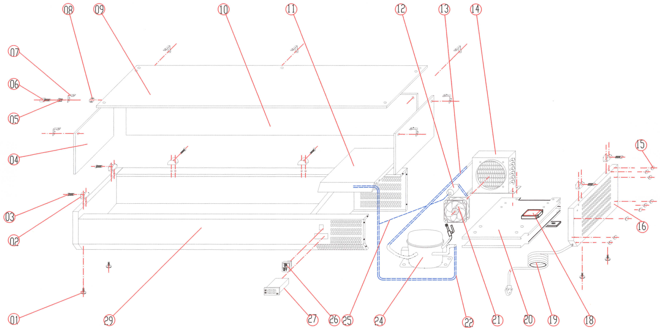
EXPLODE OF VRX1200/330
