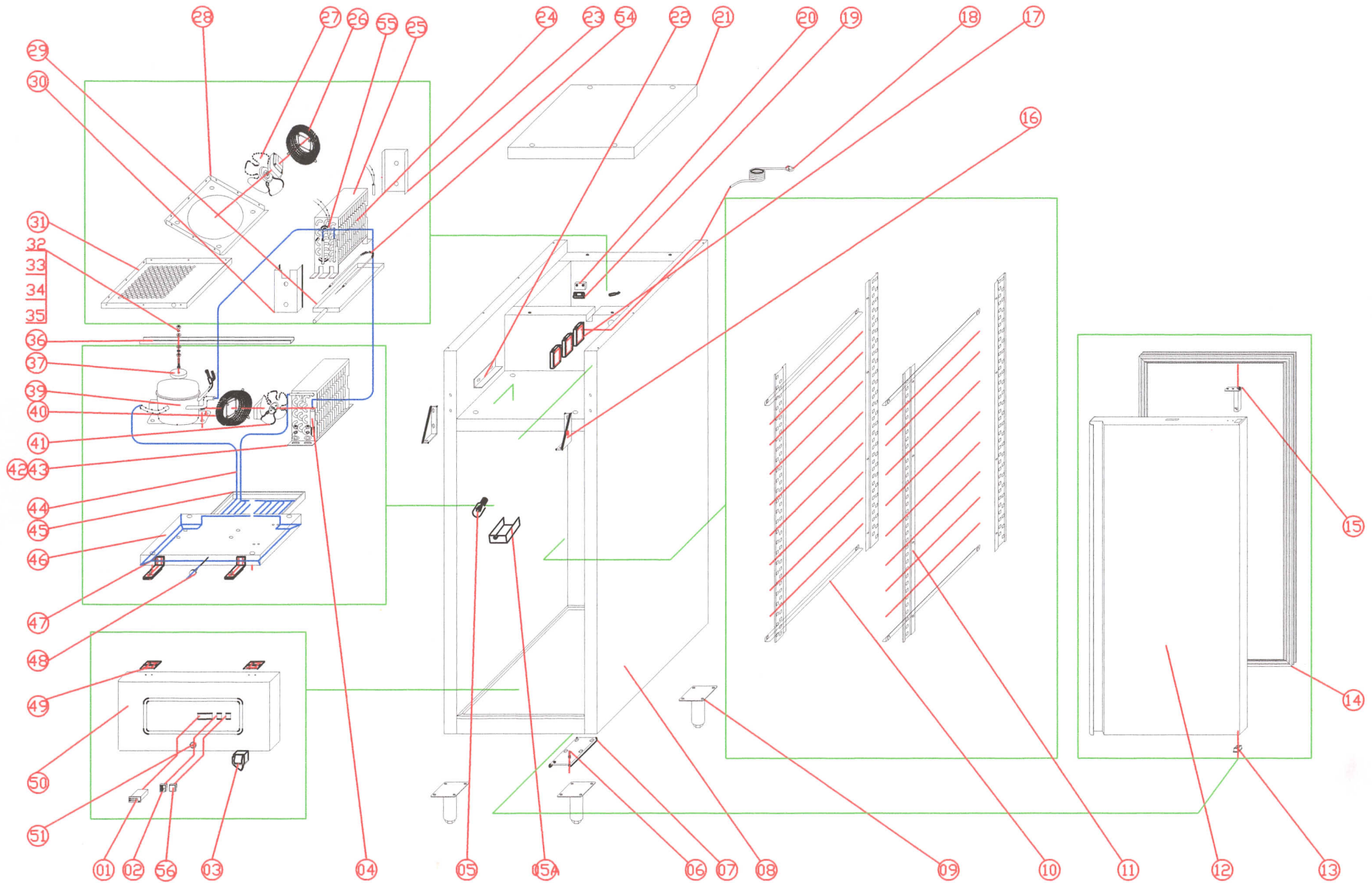
EXPLODE DIAGRAM OF PA800BT
