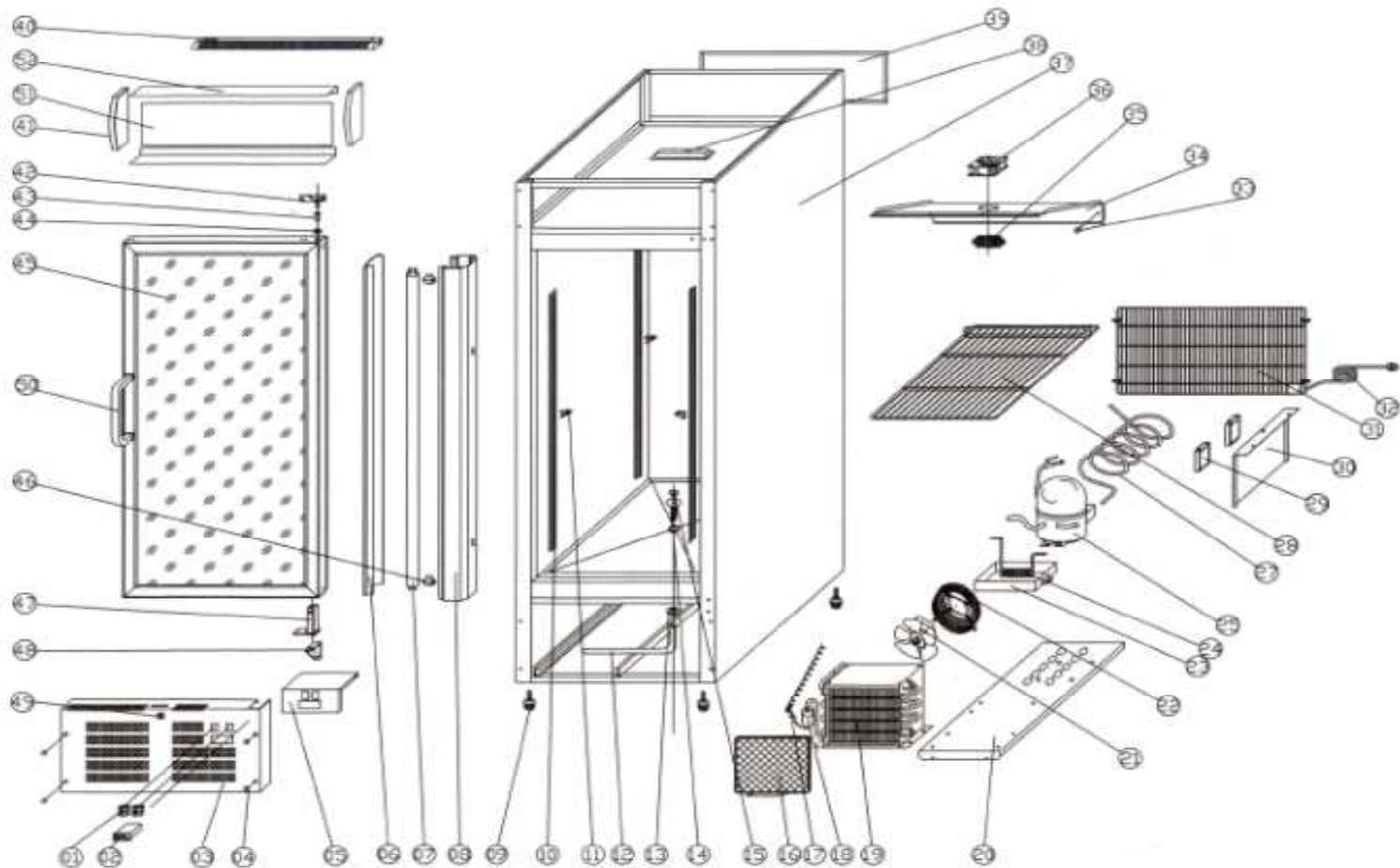
EXPLODE DIAGRAM OF SNACK340TNG
