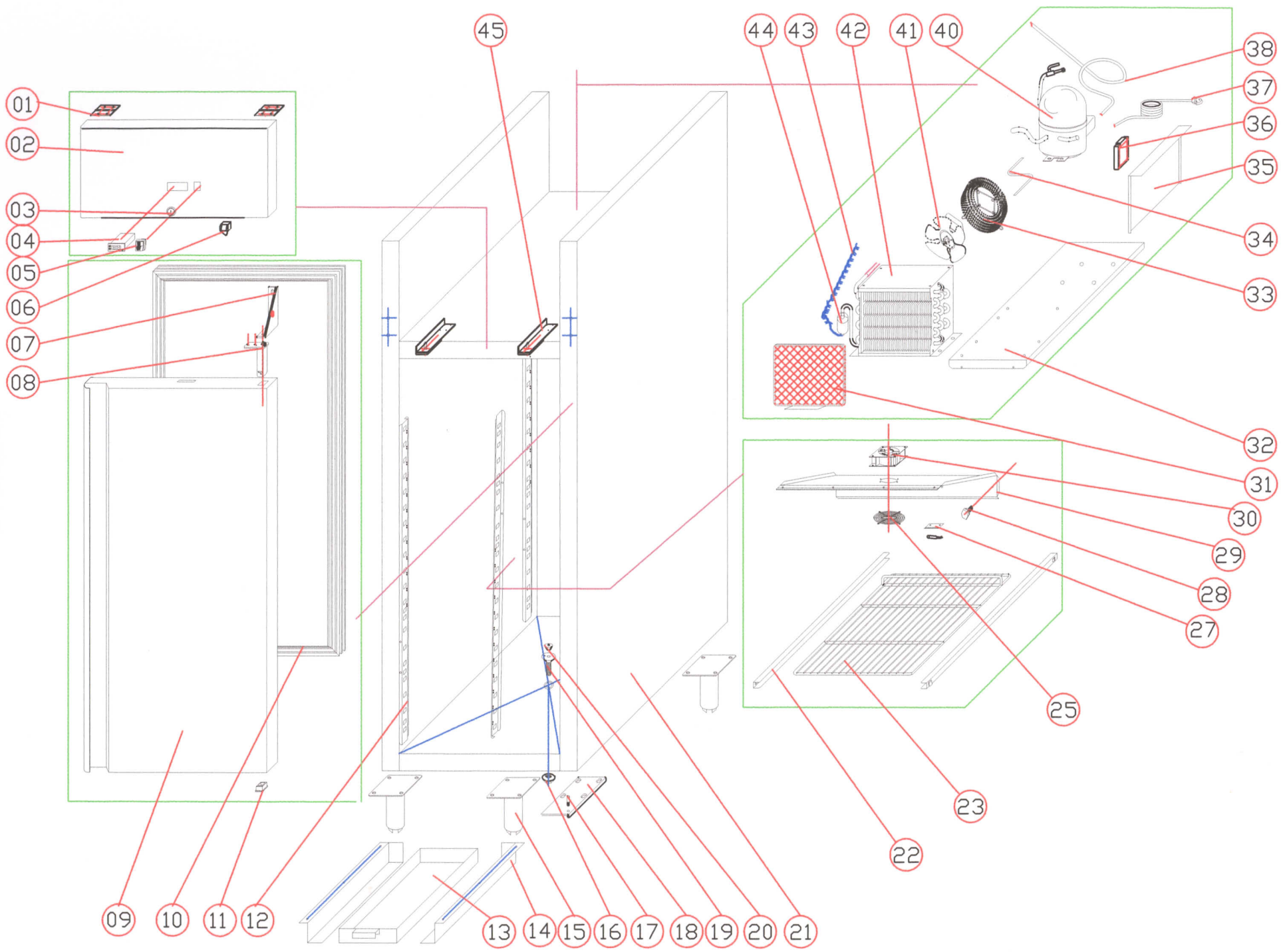
EXPLODE OF GN600TN (GN600TNZ0.6)
