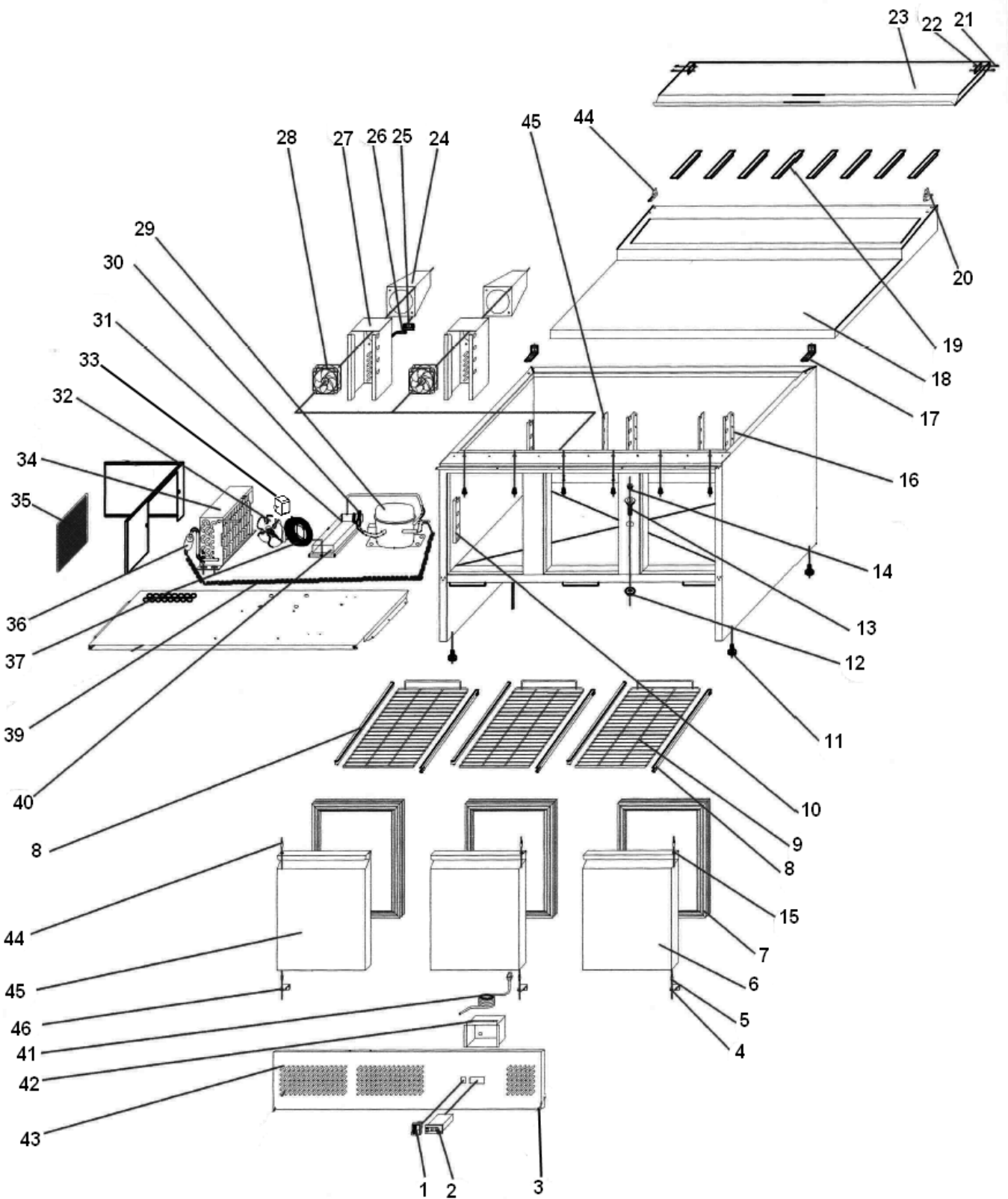
EXPLODE OF PS200-PS300
