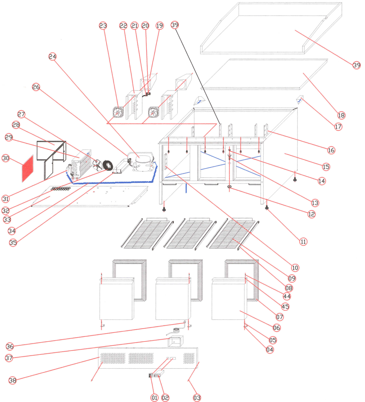
EXPLODE OF S903PZ
