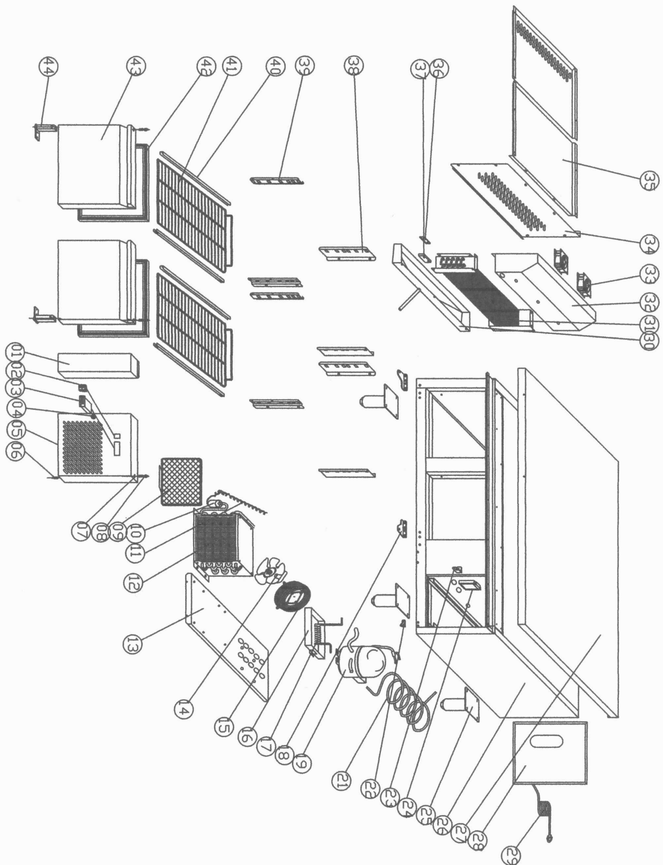
EXPLODE DF U-GN2100TN
